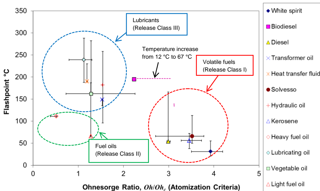
Figure 1 Classification of stakeholder fluids by flashpoint and atomisation criteria for a 10 barg release through a 1 mm diameter orifice
