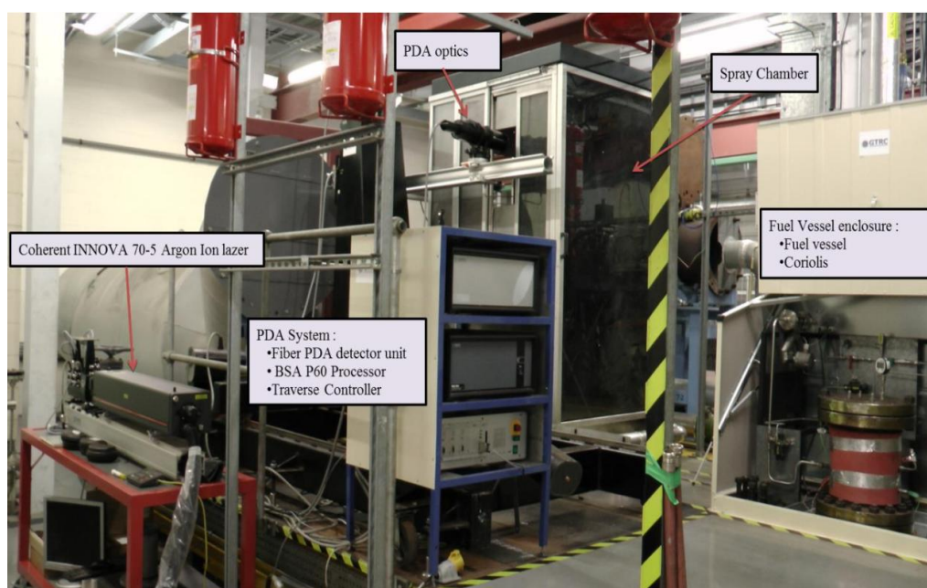
Figure 2 Photograph of test apparatus at GTRC configured for the PDA measurements
