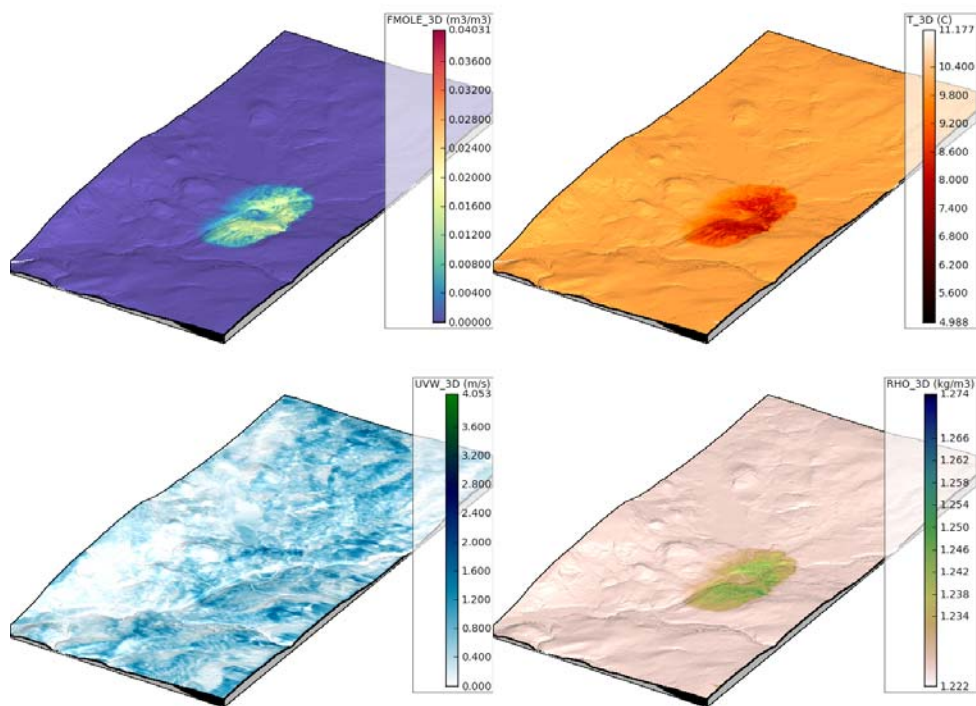
Fig. 11. Predictions of CO 2 volume fraction (v/v), temperature (°C), bulk mean velocity (m s -1 ), and density (kg m -3 ), at ground level.
