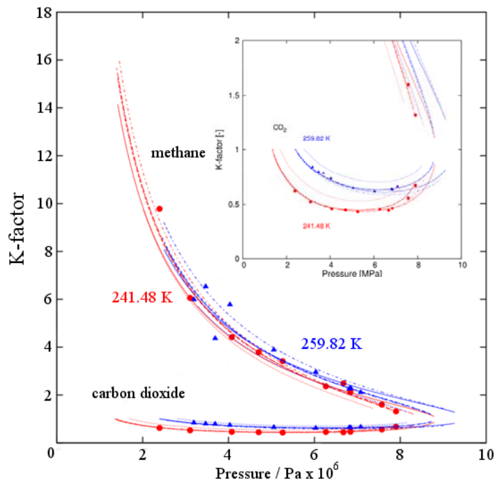
Fig. 2. K-factor ( y/x )/pressure diagram for CO 2 – CH 4 mixture. Experimental data (points) and calculations from RK ( ······ ), SRK ( - · - · - · ), PR ( - - - - - ), PR/G ( - - - - - ■ - - - - - ), SAFT ( - · - · - · ), and PC-SAFT ( ——— ). Top: predictions ( k_{ij} = 0 ), bottom: correlations ( k_{ij} \neq 0 ).
